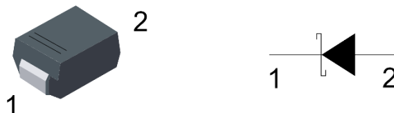
Simplified outline SMA and symbol
